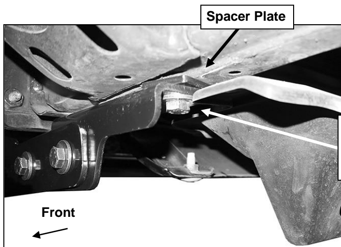
(Fig 3) Driver side pictured from below vehicle.
