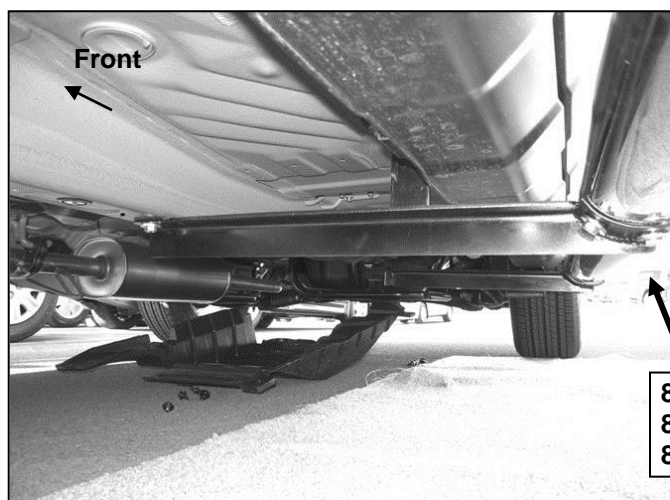
(Fig 8) Driver Side Front Mounting Bracket Pictured
