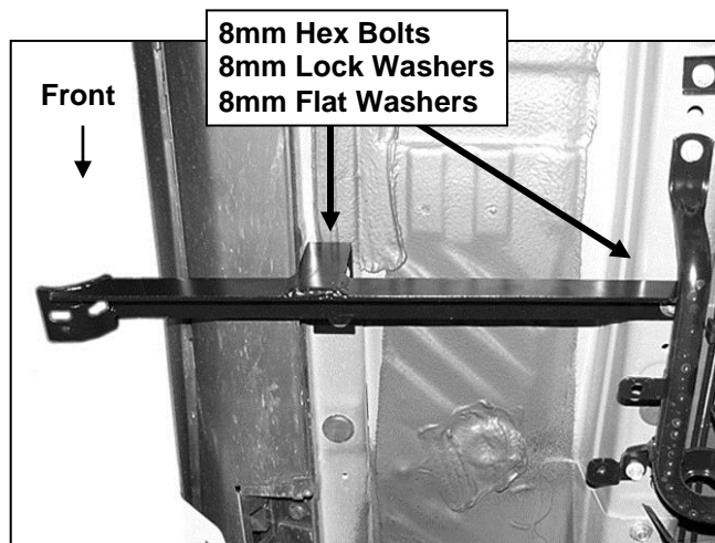
(Fig 5) Driver Side Front Mounting Bracket Pictured
