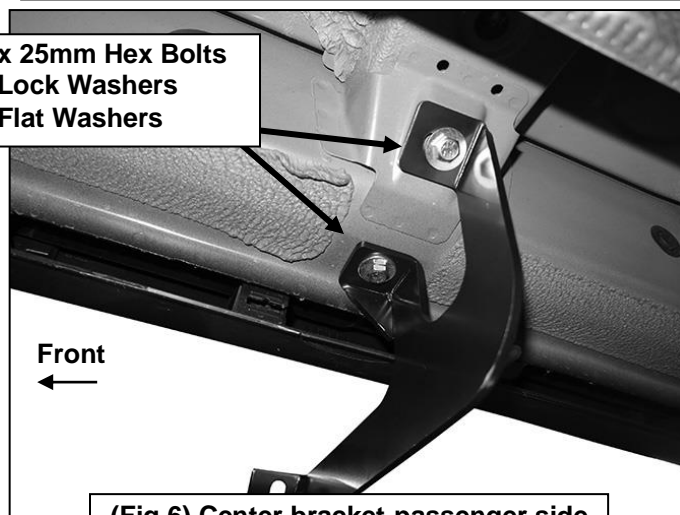
(Fig 6) Center bracket-passenger side
