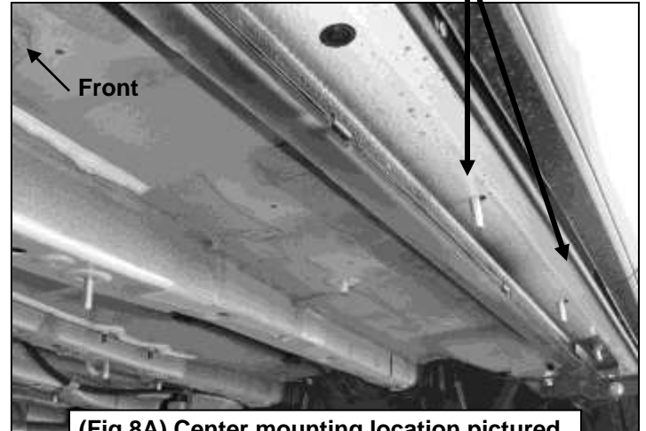
(Fig 8A) Center mounting location pictured
