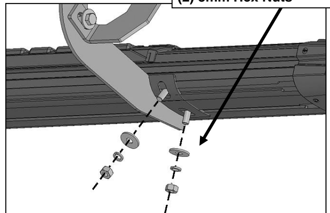
(Fig 20) Attach Sidebar to Brackets
