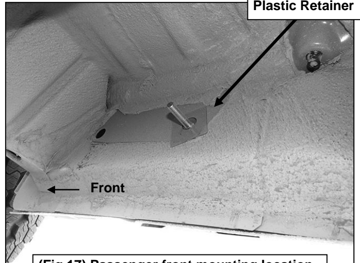
(Fig 17) Passenger front mounting location
