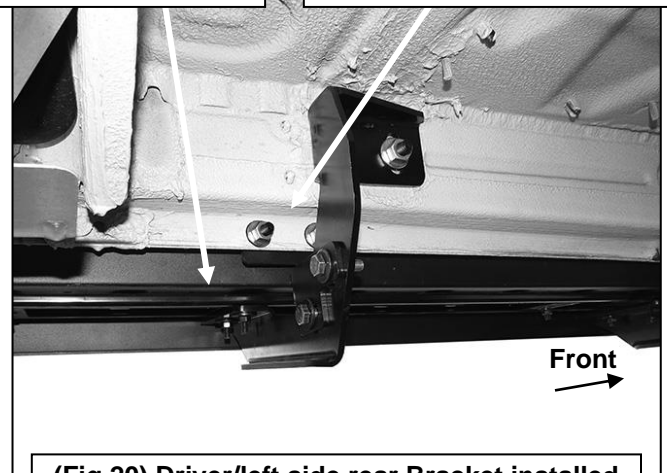
(Fig 20) Driver/left side rear Bracket installed
