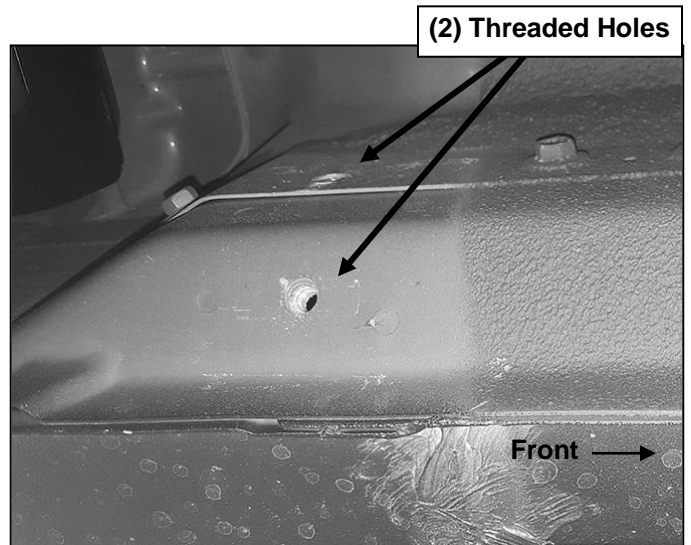
(Fig 1B) 2016-on driver side rear mounting location pictured. Note: two factory threaded holes only
