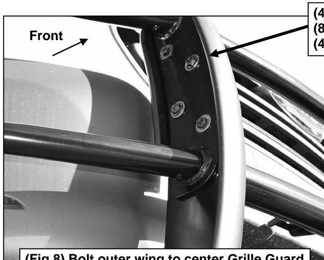
(Fig 8) Bolt outer wing to center Grille Guard (Passenger side installation pictured)
