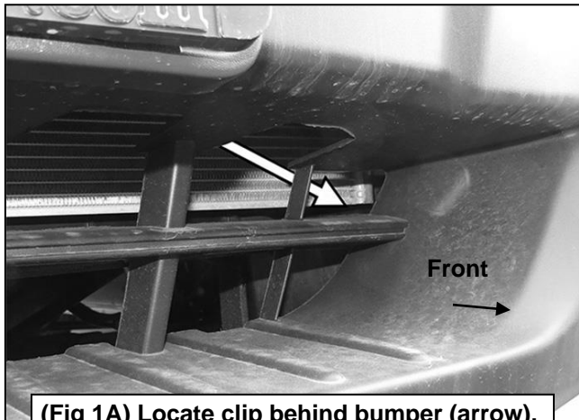
(Fig 1A) Locate clip behind bumper (arrow), at each end of bumper opening
