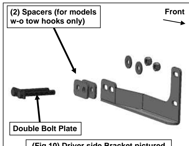
(Fig 10) Driver side Bracket pictured
