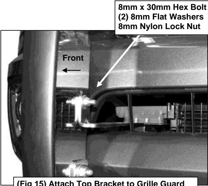
(Fig 15) Attach Top Bracket to Grille Guard
