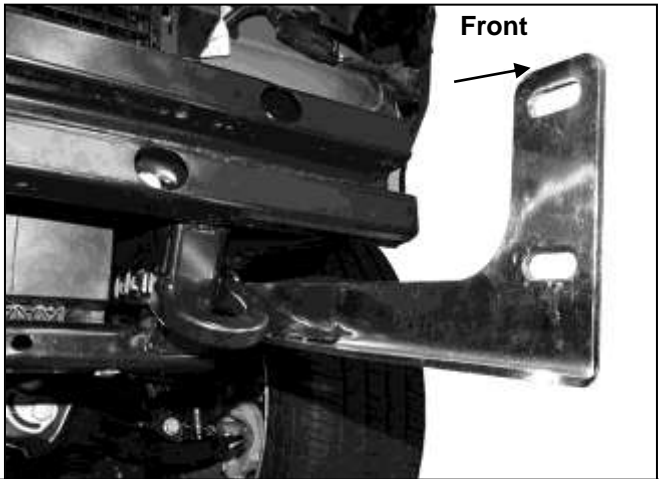
(Fig 13) Driver side Bracket installed over tow hook, Spacers are not required. Installation pictured without bumper for instruction purposes only
