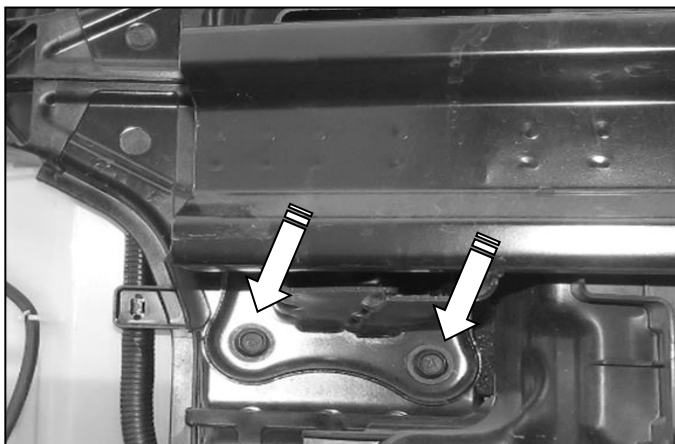
(Fig 5) Remove three bolts from the original car anti-collision beam on the left and right sides.
