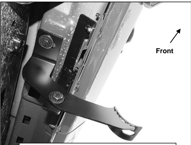
(Fig 6) Driver/left front Brackets installed
