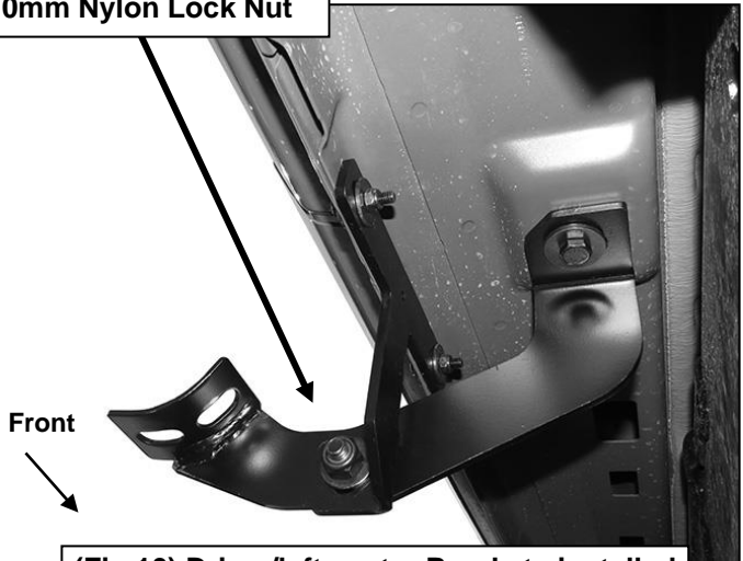
(Fig 10) Driver/left center Brackets installed
