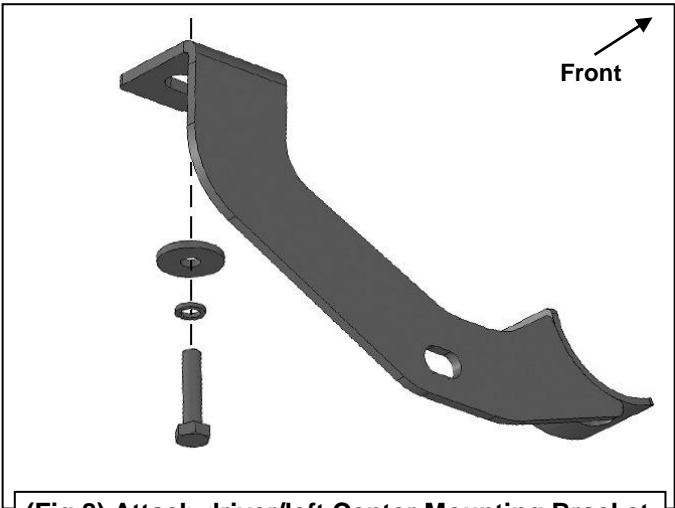
(Fig 8) Attach driver/left Center Mounting Bracket
