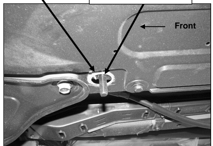
(Fig 2B) Driver side front inner mounting location
