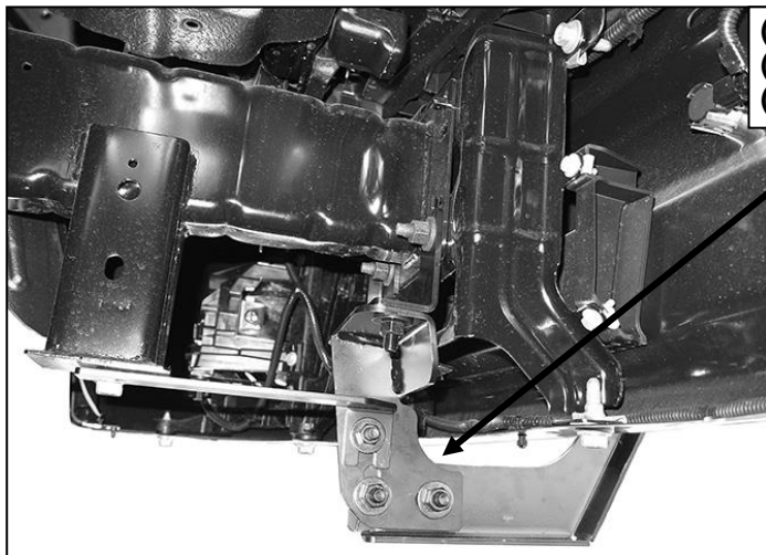
(Fig 17) Attach Bull Bar assembly to Mounting Bracket
