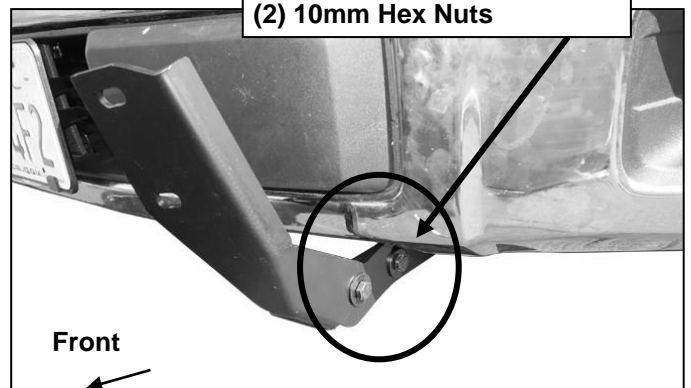
(Fig 9) Driver side Frame Bracket attached to Bull Bar Bracket Pictured
