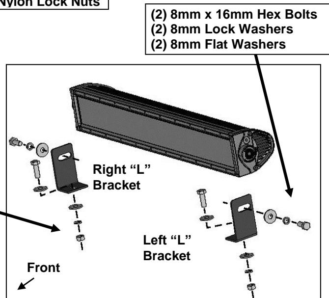
(Fig 15) Typical center light installation
