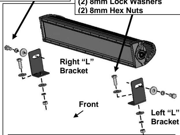
(Fig 8) Example of center light installation
