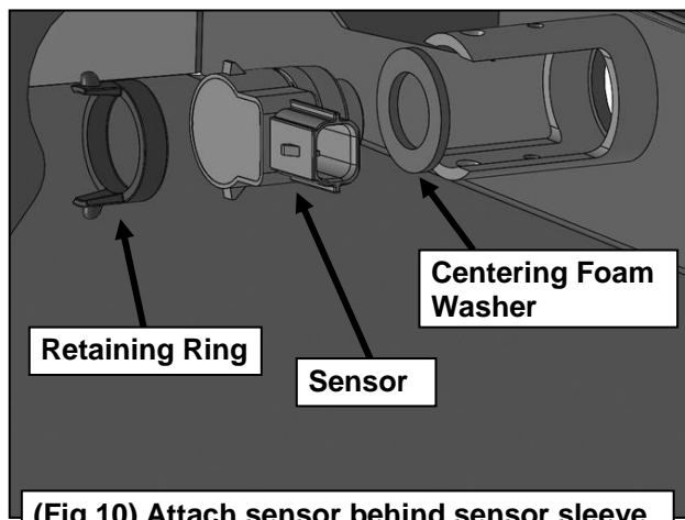
(Fig 10) Attach sensor behind sensor sleeve
