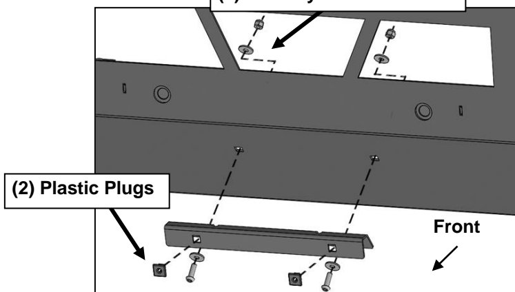
(Fig 11) Attach License Plate Bracket to Bumper
