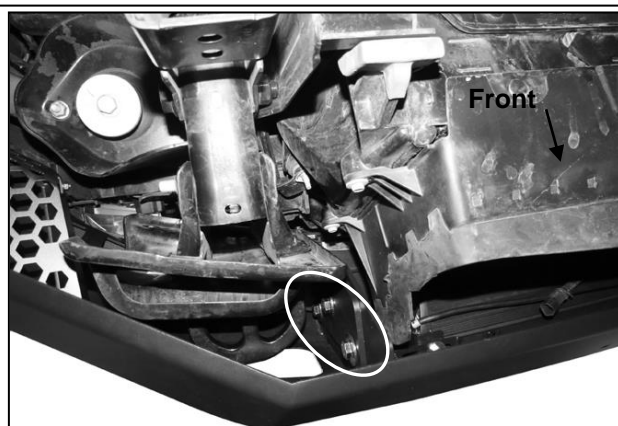
(Fig 13) Driver/left side complete installation (pictured from below Bumper)
