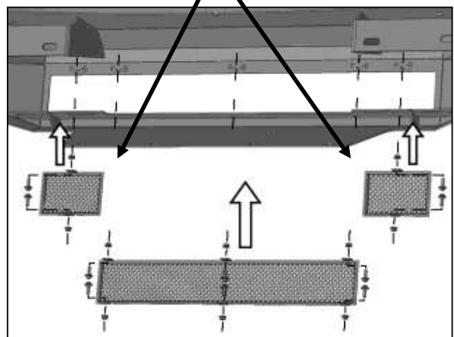
(Fig 16) Attach Inner and Center Mesh Plates to tabs on the back of the bumper as desired
