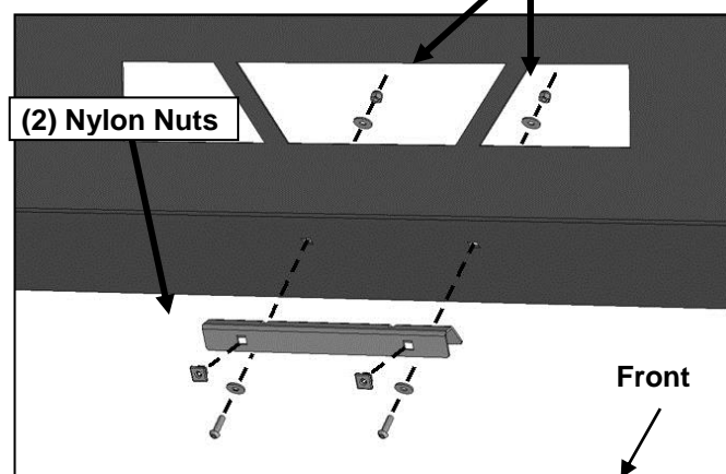
(Fig 12) Attach License Plate Bracket to Bumper
