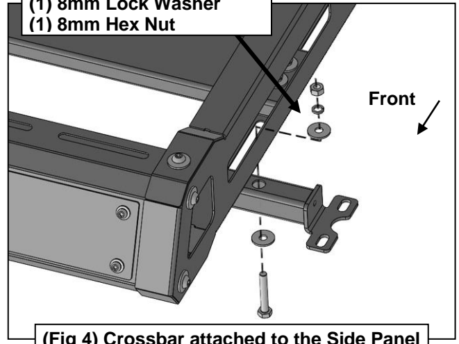
(Fig 4) Crossbar attached to the Side Panel
