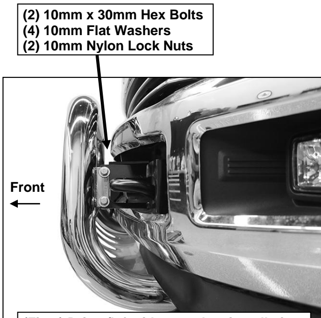
(Fig 7) Driver/left side complete installation
