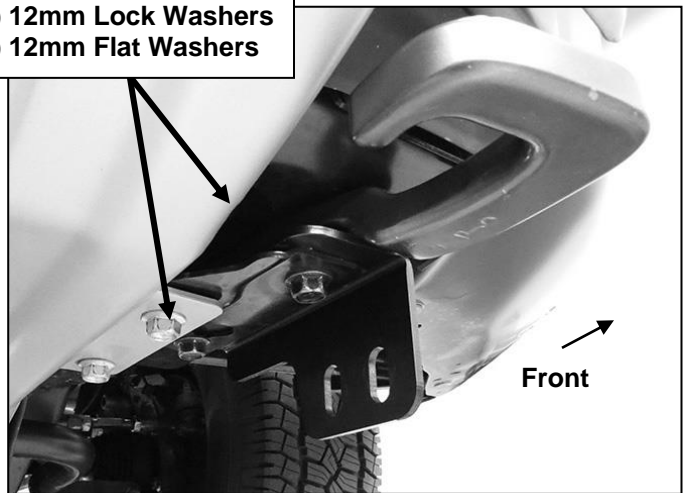
(Fig 2) Attach Frame Bracket to tow hook. Replace hardware with supplied longer 12mm Fine Thread Hex Bolts, Lock Washers and Flat Washers.
