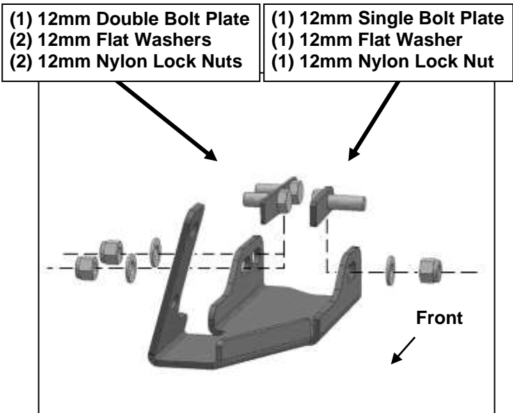
(Fig 6) Passenger/right side Bracket illustrated
