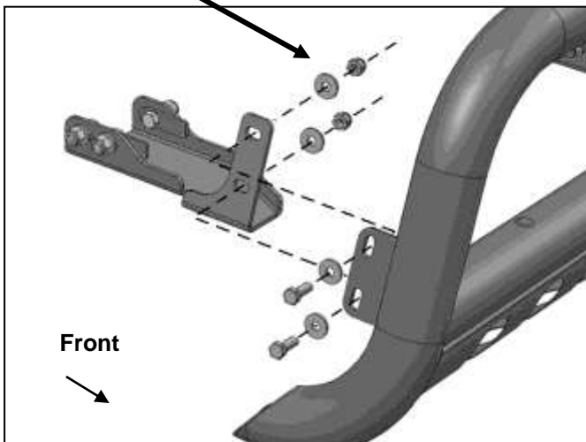
(Fig 13) Attach Bull Bar to outside of Brackets. Passenger/right side complete installation
