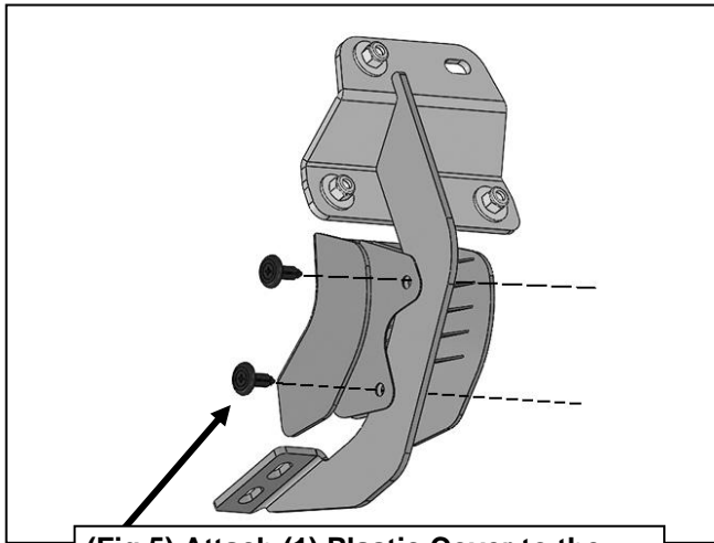
(Fig 5) Attach (1) Plastic Cover to the Mounting Bracket with (2) Plastic Clips
