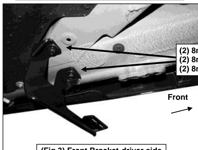
(Fig 3) Front Bracket-driver side
