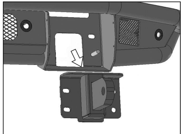
(Fig 2) Remover driver/left Shackle Mounting Bracket.
