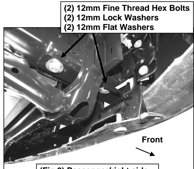
(Fig 2) Passenger/right side Mounting Bracket installed
