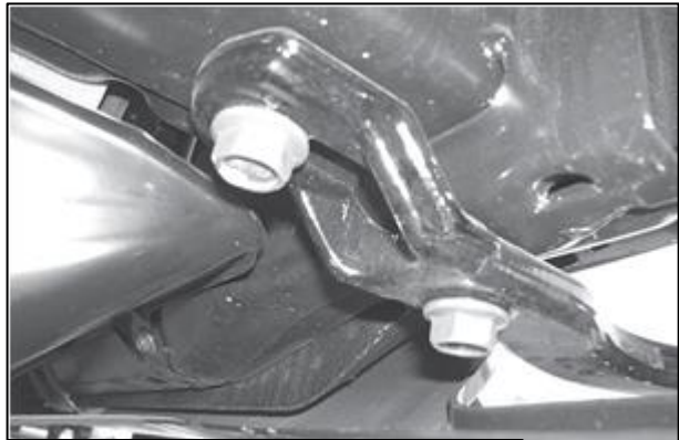
(Fig 2) Remove tow hooks if equipped, (passenger/right tow hook pictured)
