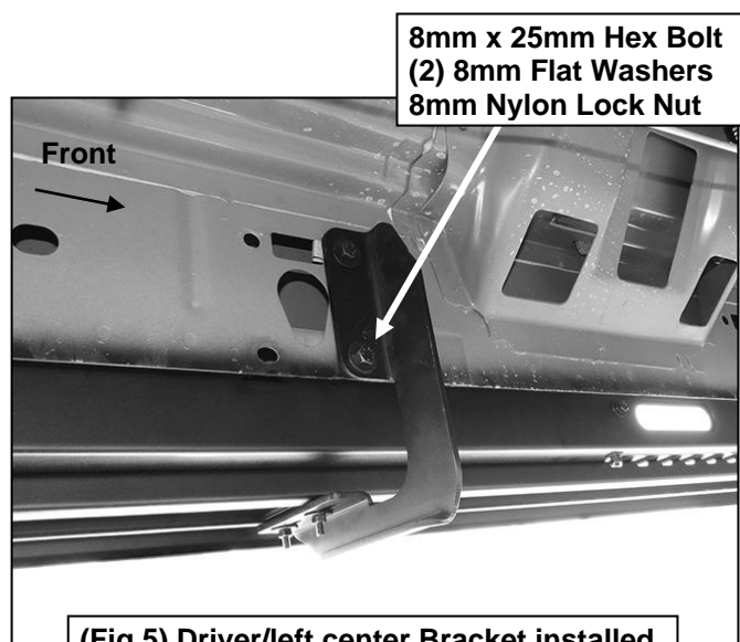
(Fig 5) Driver/left center Bracket installed
