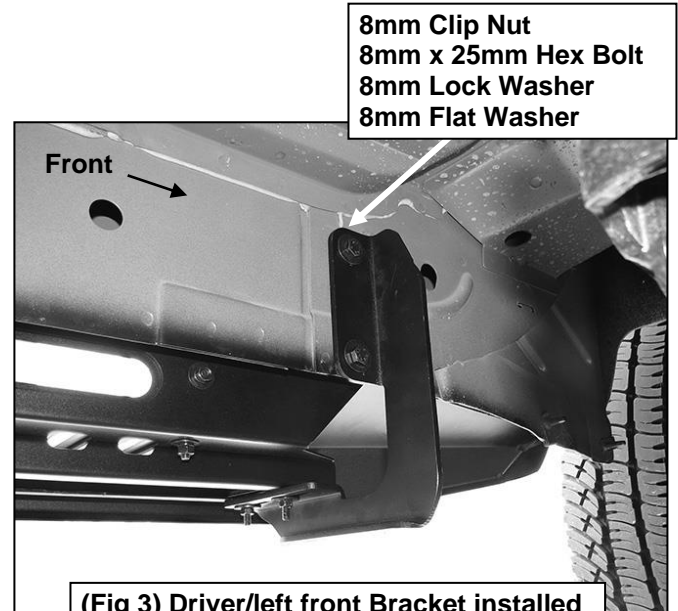
(Fig 3) Driver/left front Bracket installed
