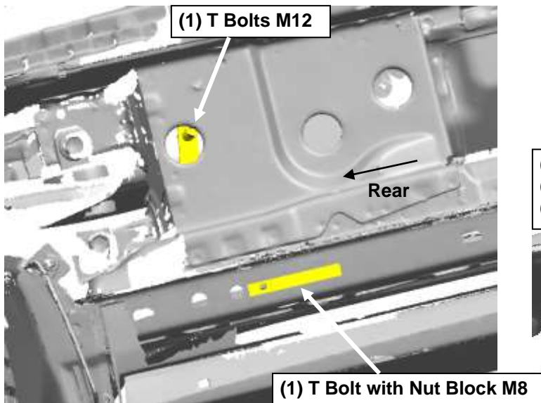
(Fig 4) Mounting position of Rear Bracket
