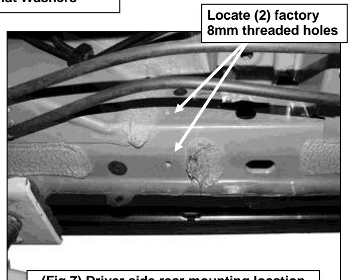
(Fig 7) Driver side rear mounting location
