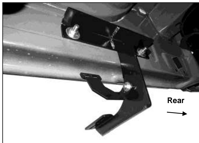
(Fig 18) Passenger rear Mounting Bracket assembly
