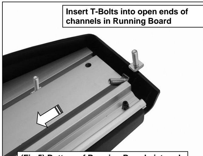
(Fig 5) Bottom of Running Board pictured
