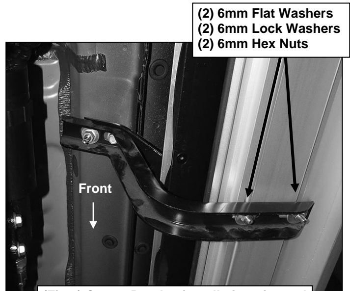
(Fig 6) Center Bracket installation pictured
