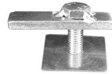
(Fig 2) 10mm Bolt Plate w-retainer
