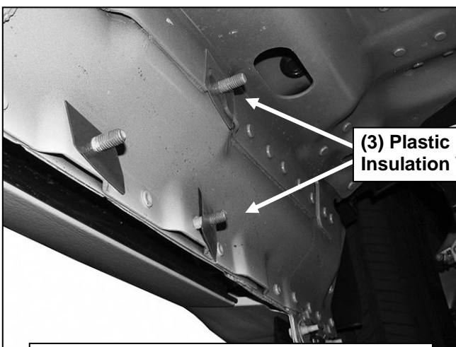
(Fig 3) Thread Plastic Washers onto all mounting studs. Driver side front pictured
