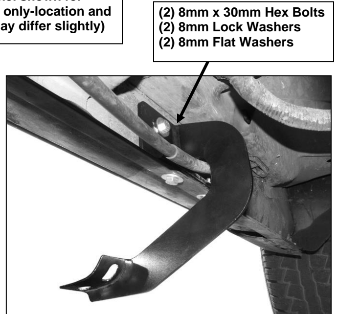
(Fig 2) Driver side-front Mounting Bracket location
