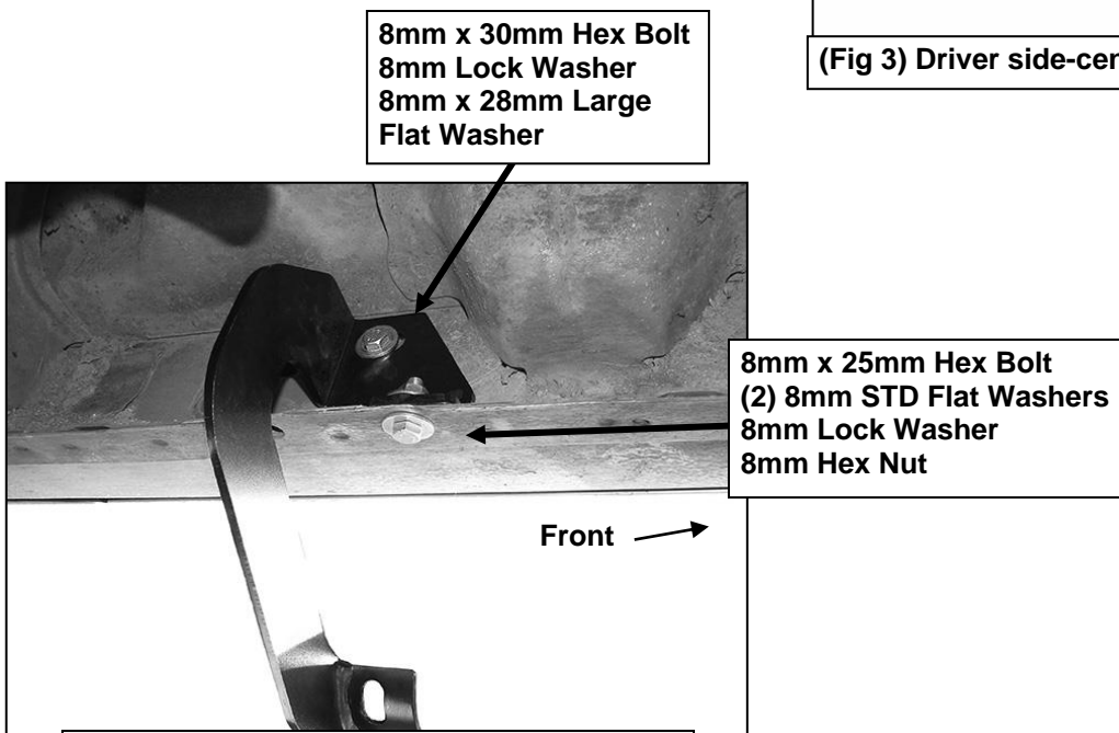
(Fig 4) Driver Side Center Bracket installed
