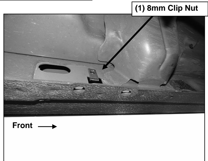
(Fig 3) Driver side-center Mounting Bracket location
