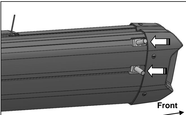
(Fig 13) Insert 8mm T-Bolts through the channel openings in the bottom of the Sidebar
