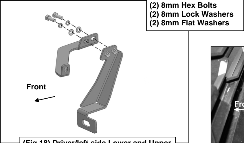
(Fig 18) Driver/left side Lower and Upper Bracket Assembled above
