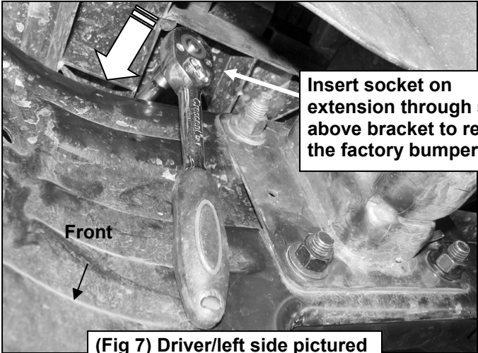
(Fig 7) Driver/left side pictured
