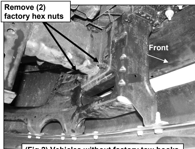
(Fig 2) Vehicles without factory tow hooks
