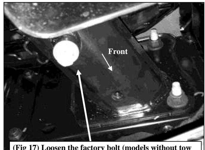
(Fig 17) Loosen the factory bolt (models without tow hooks pictured on the passenger/right side)
