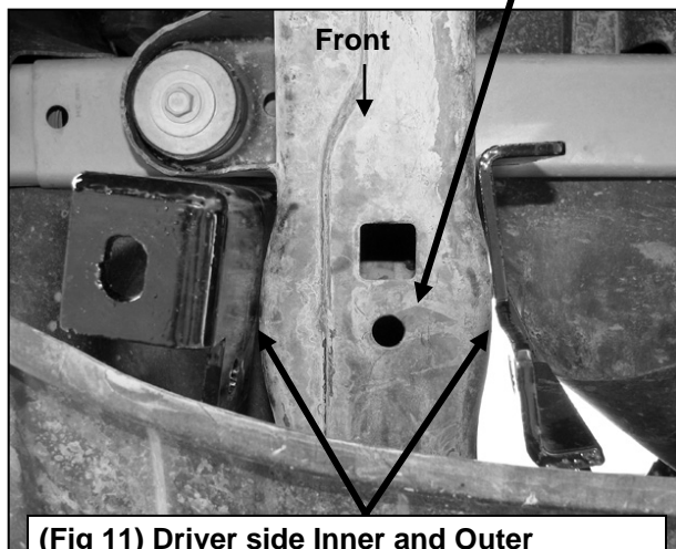
(Fig 11) Driver side Inner and Outer Support Brackets pictured from below. Note fit of Brackets against frame channel
