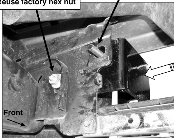
(Fig 6) Driver side viewed from behind bumper
