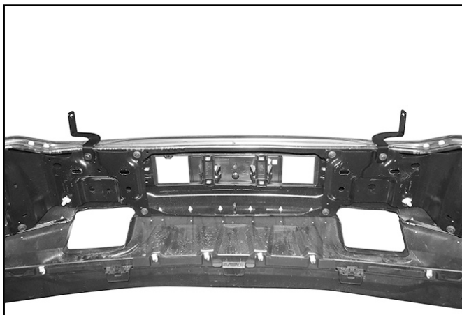
(Fig 22) 2018 models: Top Support Brackets attached to bumper
