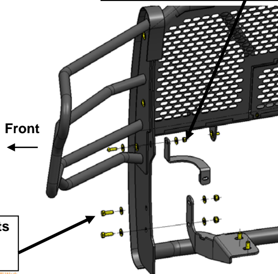
(Fig 25) 2018 models: Complete installation
