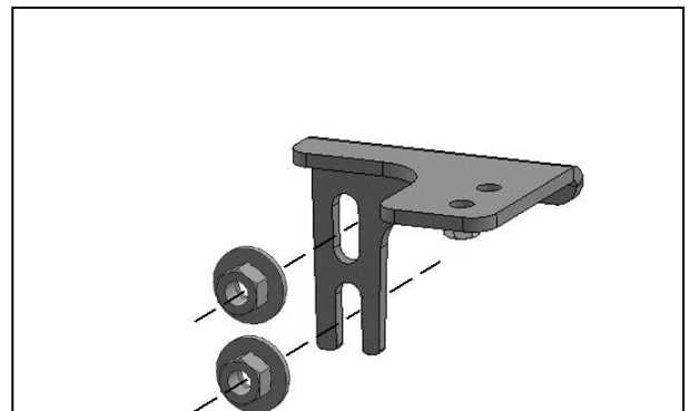
(Fig 3A) Reuse the (2) factory hex nuts to attach the passenger/right Top Bracket to the factory bumper bracket
