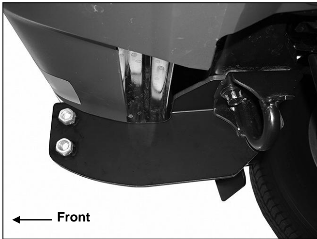
(Fig 8B) Install Frame Bracket with factory tow hook bolts. Small tow hook pictured FOR EXAMPLE ONLY
