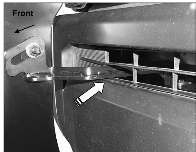
(Fig 9B) Insert Top Bracket into opening in bumper (Grille guard pictured installed for reference only do not install at this time)
