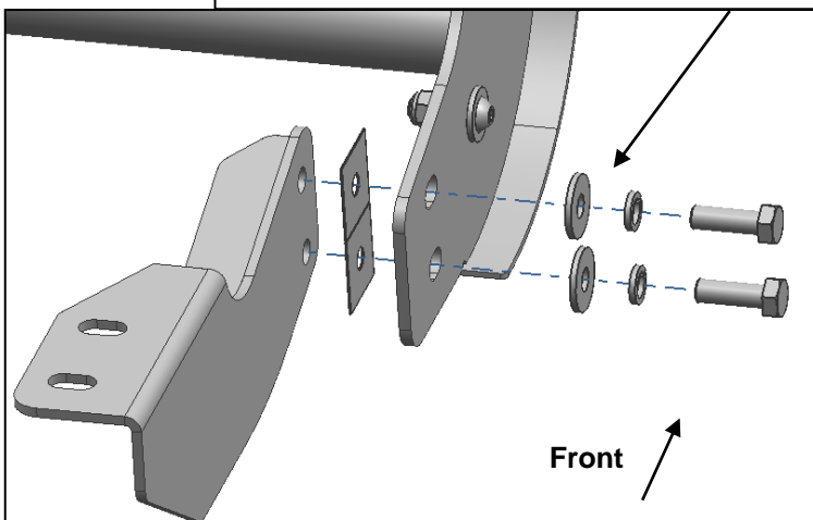
(Fig 11) Insert a Plastic Washer between the Grille Guard and the Frame Mounting Bracket on each 12mm Hex Bolt
