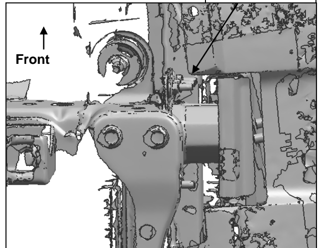
(Fig 4) Reuse factory hex nuts to secure Top Bracket to end of frame. Remove tow hooks
