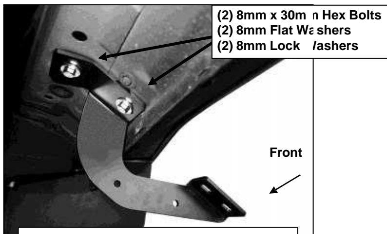
(Fig 3) Passenger front Bracket installation
