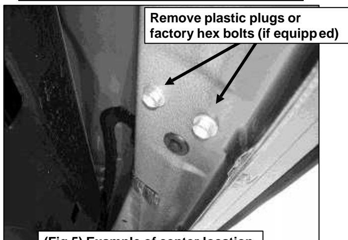
(Fig 5) Example of center location
