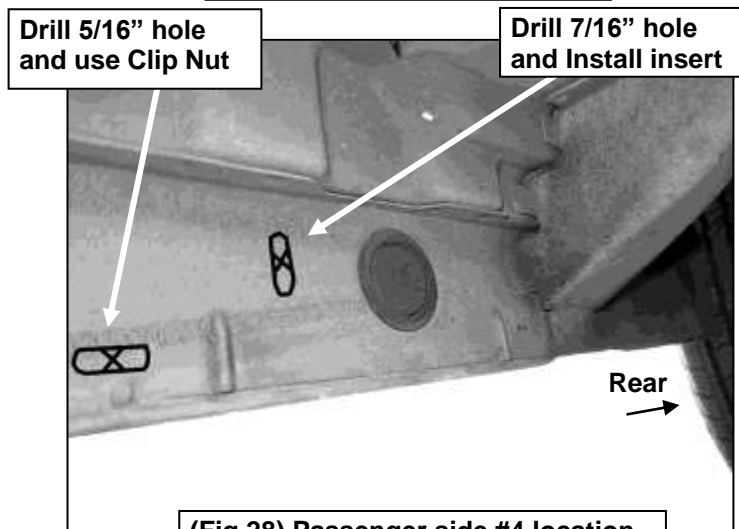
(Fig 28) Passenger side #4 location
