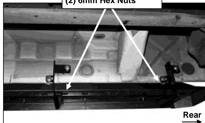
(Fig 33) Passenger/right #4 and #5, (rear), Bracket installation pictured. NOTE #4 and #5 Brackets are identical.
