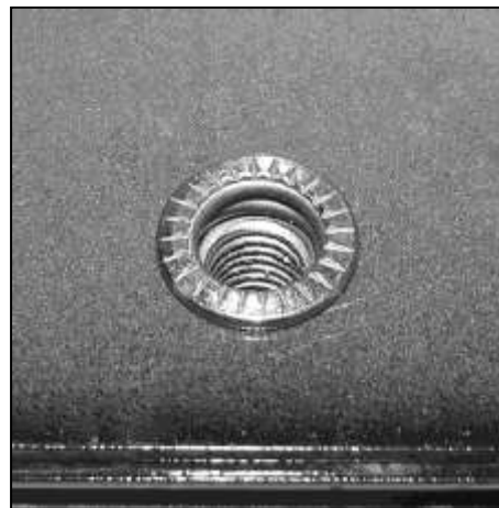
(Fig 31) Example fully installed Insert
