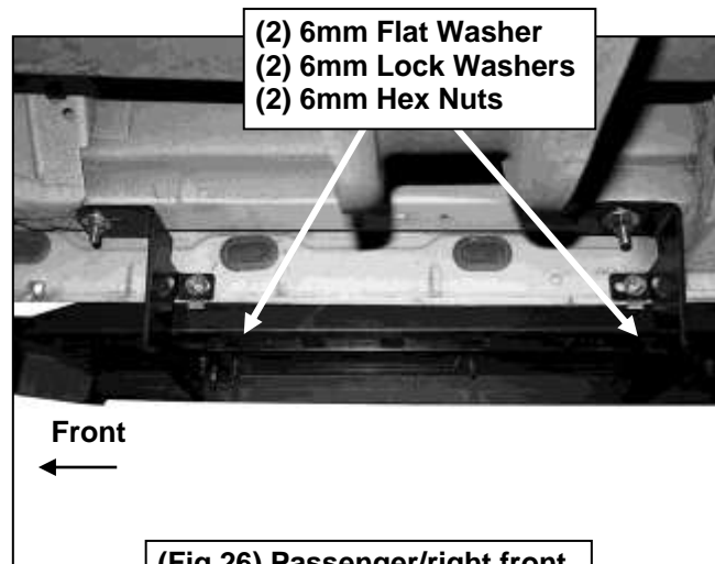
(Fig 26) Passenger/right front and #2 Bracket installation
