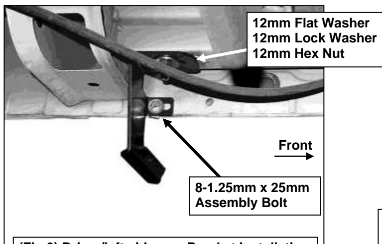
(Fig 9) Driver/left side rear Bracket installation
