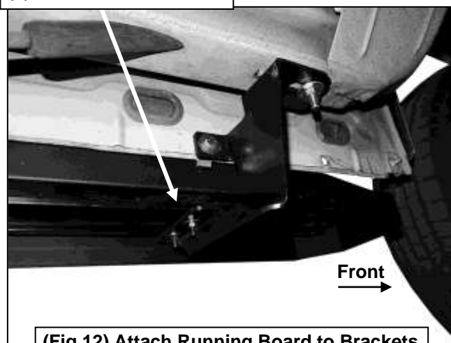
(Fig 12) Attach Running Board to Brackets
