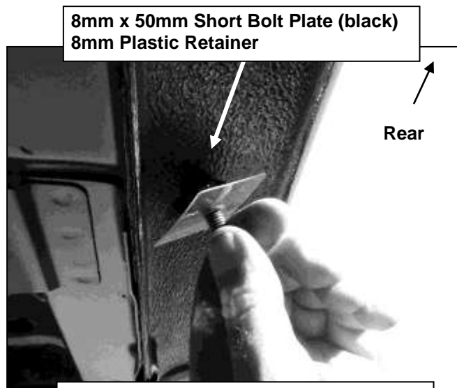
(Fig 8) Slide 8mm x 50mm Short Bolt Plate into outer hole in body panel
