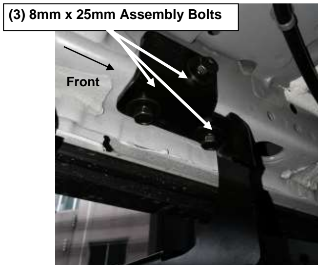
(Fig 5) Driver /Left Rear Mounting Bracket Pictured
